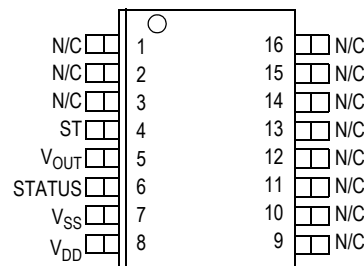
Figure 2. Pin Connections
